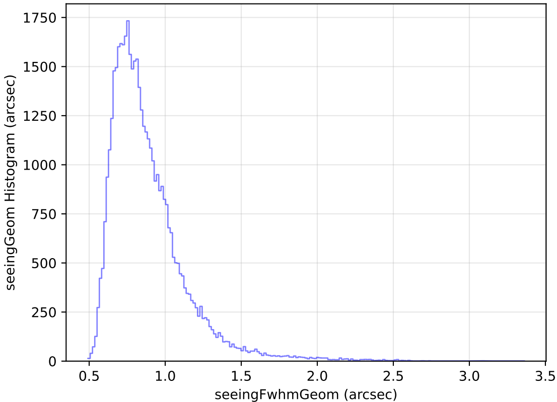
too_ignore_100_1v3.4_10yrs Yr 1 z band: seeingGeom Histogram
