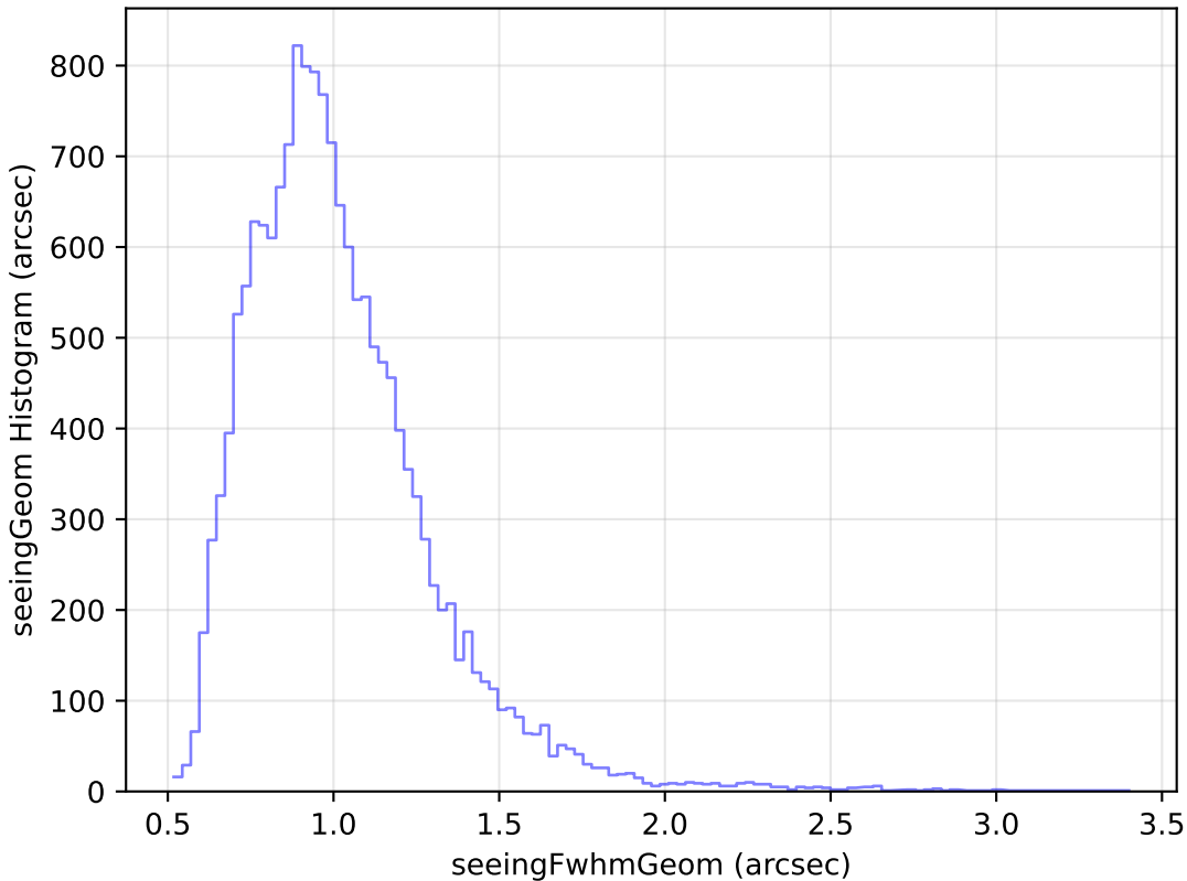
too_ignore_100_1v3.4_10yrs Yr 1 u band: seeingGeom Histogram
