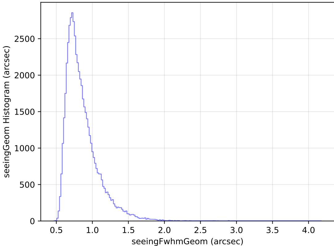
too_ignore_100_1v3.4_10yrs Yr 1 i band: seeingGeom Histogram
