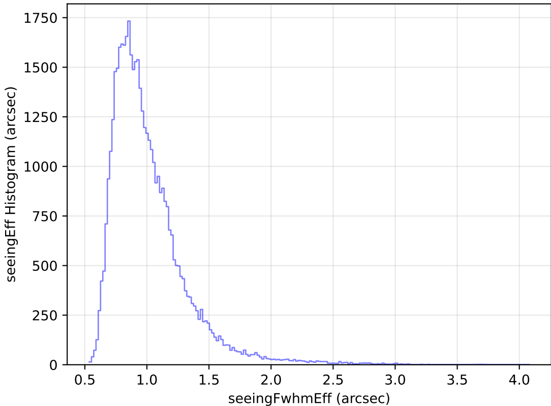
too_ignore_100_1v3.4_10yrs Yr 1 z band: seeingEff Histogram
