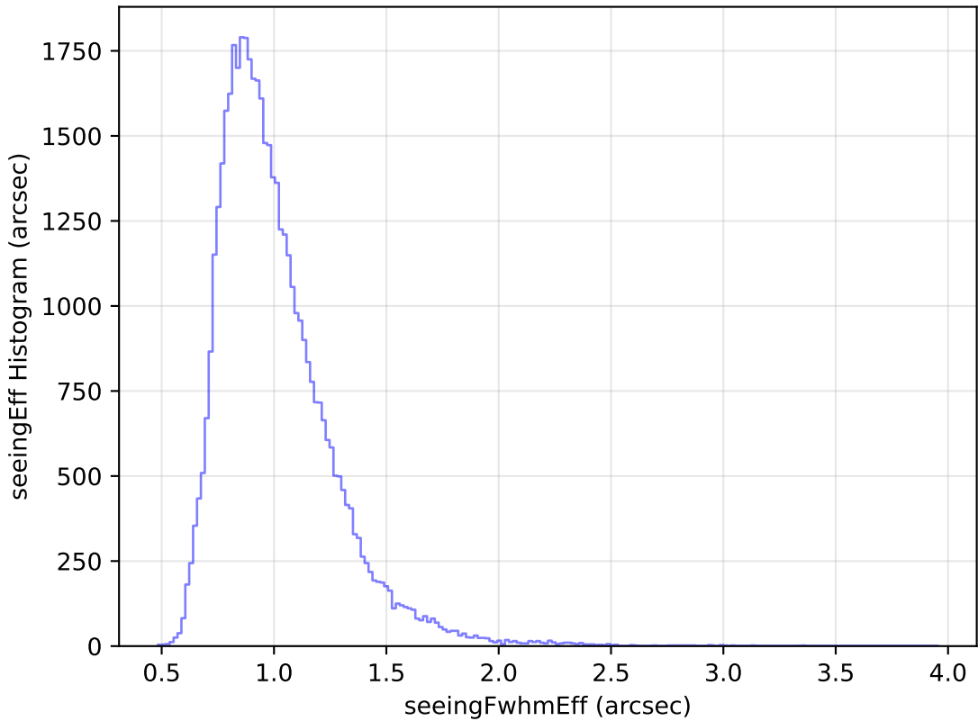
too_ignore_100_1v3.4_10yrs Yr 1 y band: seeingEff Histogram
