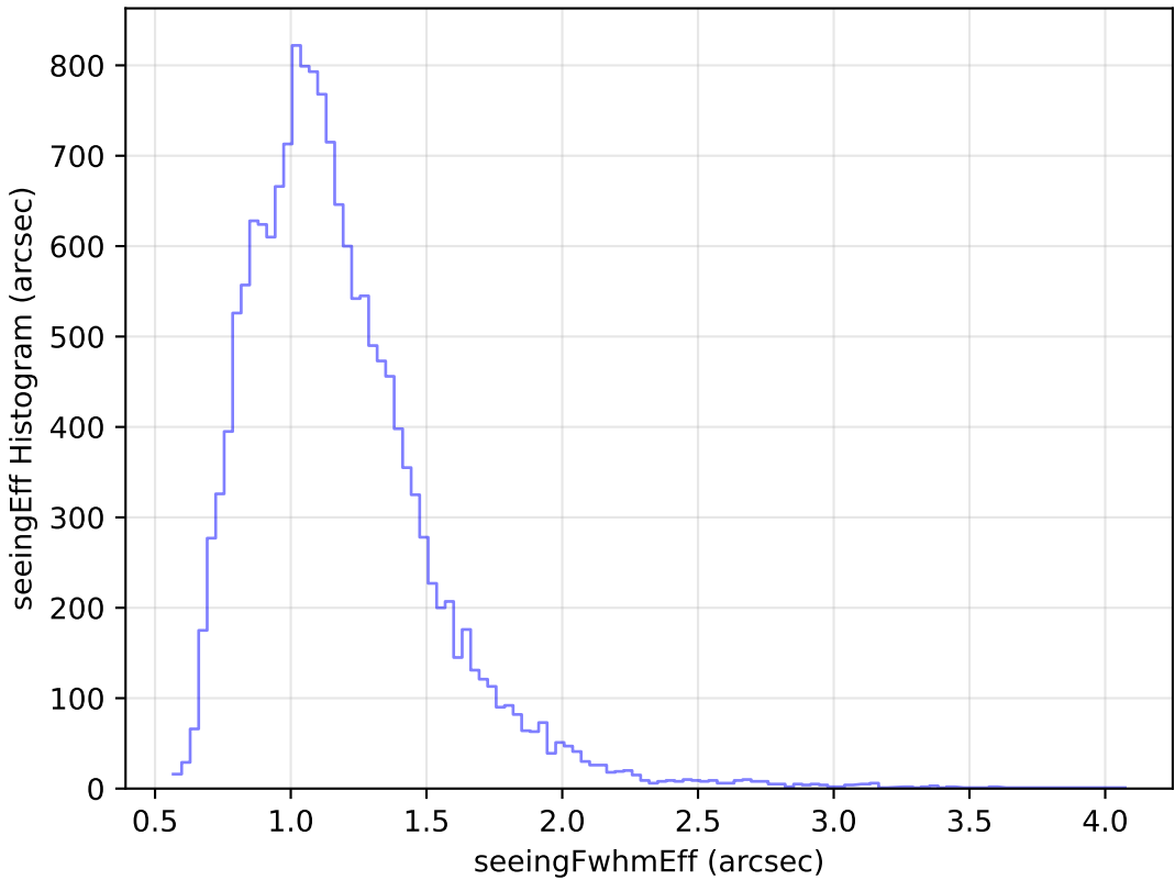
too_ignore_100_1v3.4_10yrs Yr 1 u band: seeingEff Histogram
