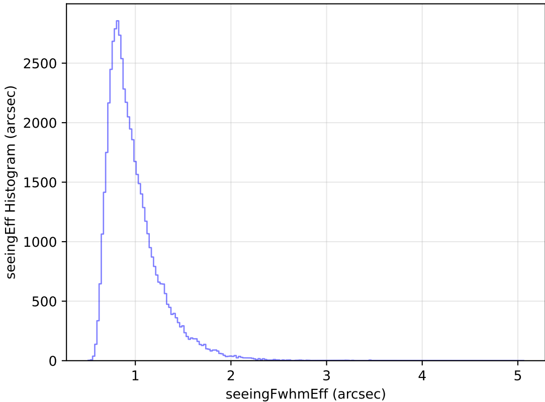
too_ignore_100_1v3.4_10yrs Yr 1 i band: seeingEff Histogram
