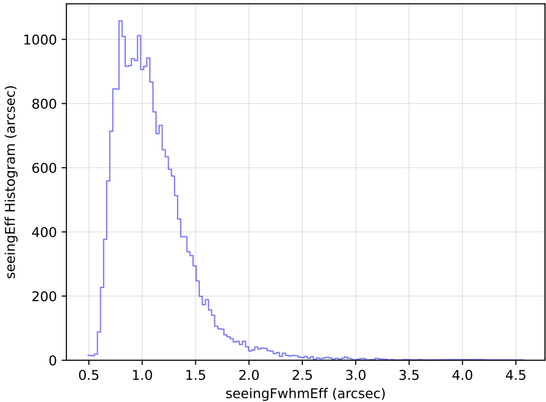
too_ignore_100_1v3.4_10yrs Yr 1 g band: seeingEff Histogram
