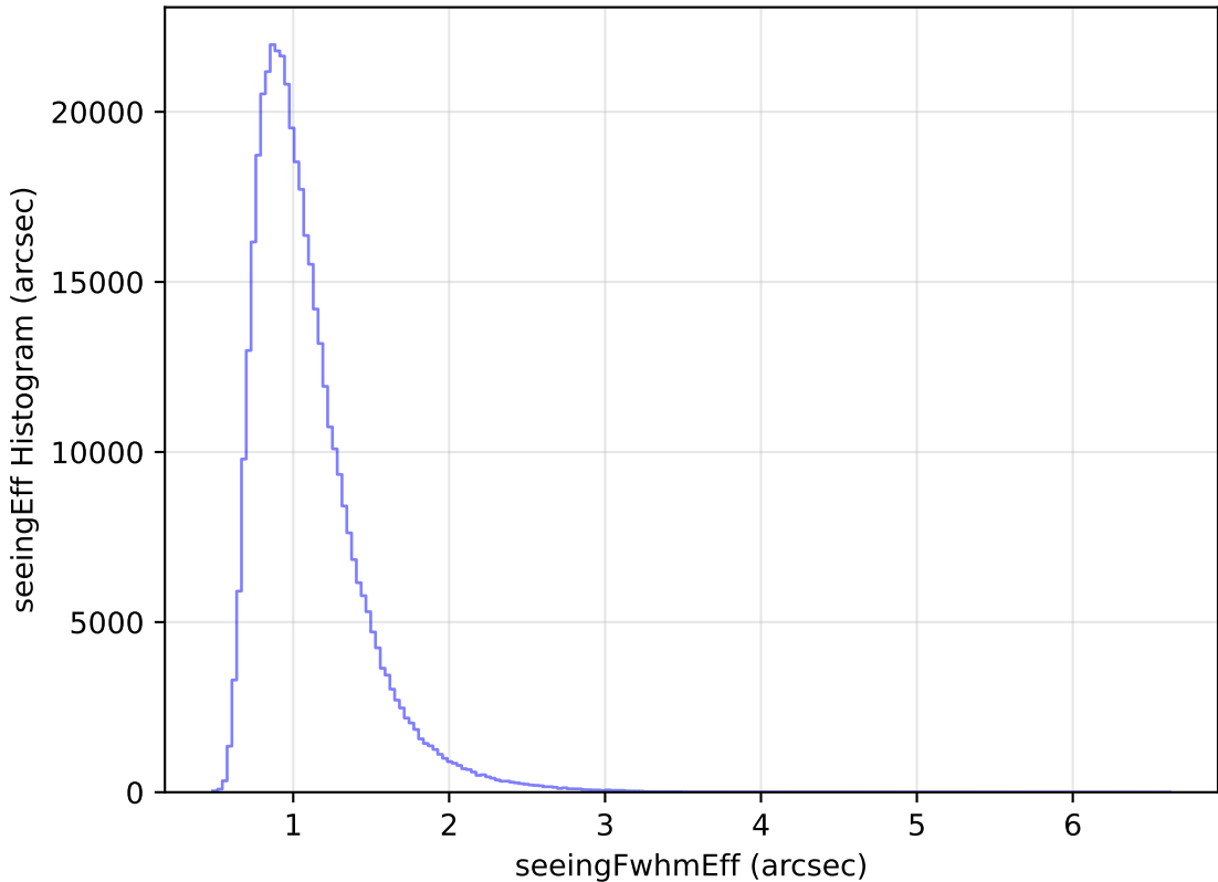
too_ignore_100_1v3.4_10yrs WFD z band: seeingEff Histogram
