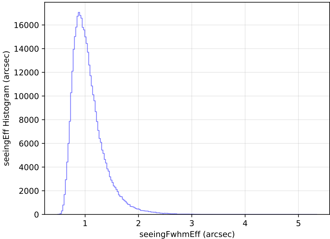
too_ignore_100_1v3.4_10yrs WFD y band: seeingEff Histogram
