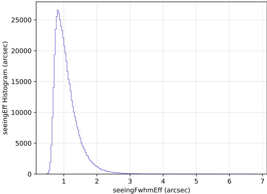
too_ignore_100_1v3.4_10yrs WFD i band: seeingEff Histogram
