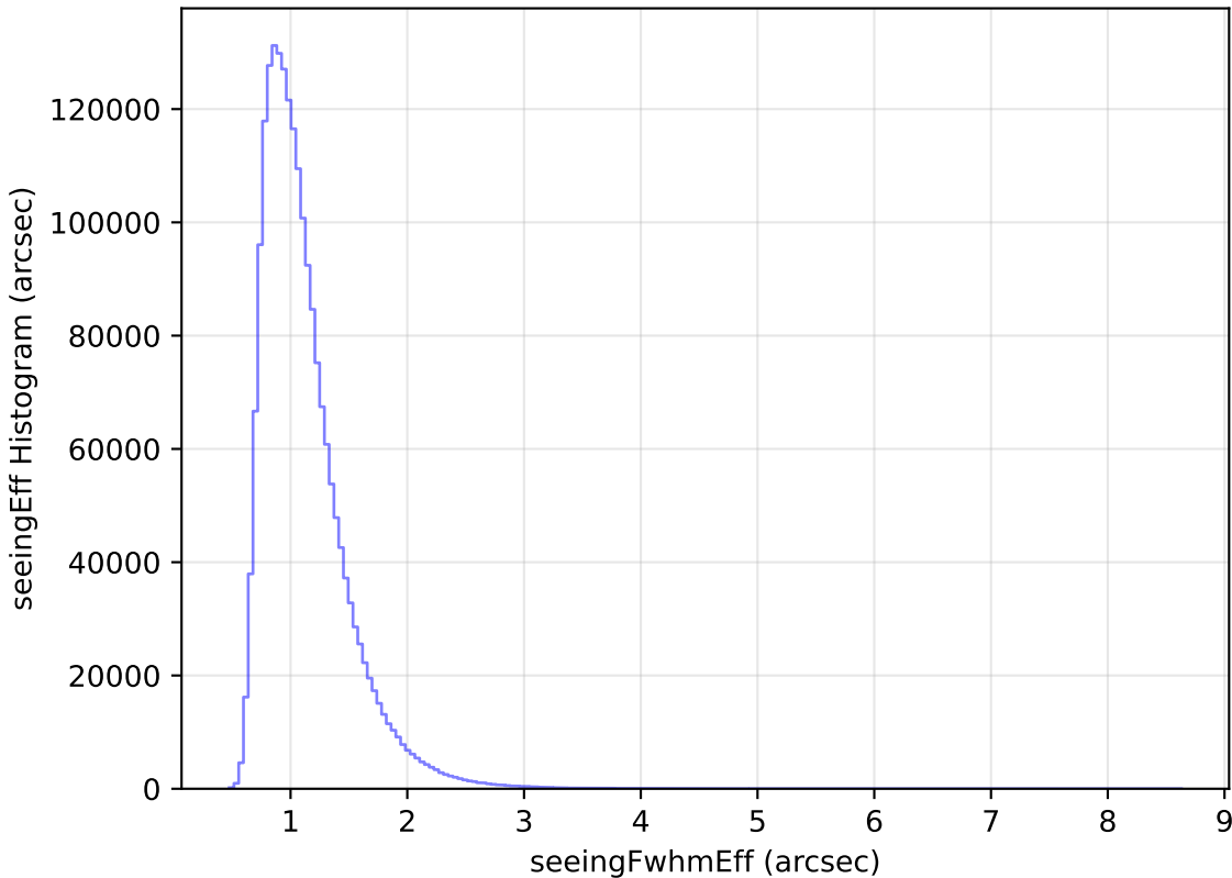
too_ignore_100_1v3.4_10yrs WFD all bands: seeingEff Histogram
