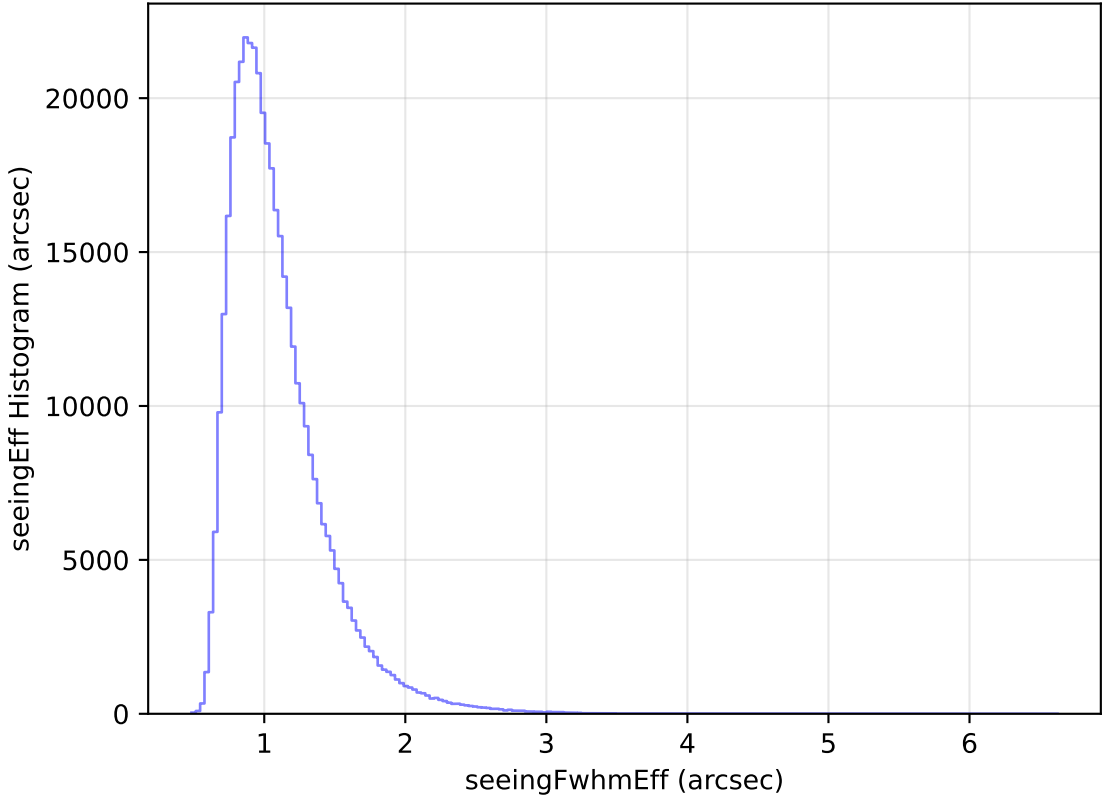
too_ignore_100_1v3.4_10yrs All sky z band: seeingEff Histogram
