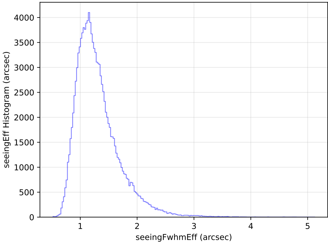
too_ignore_100_1v3.4_10yrs All sky u band: seeingEff Histogram
