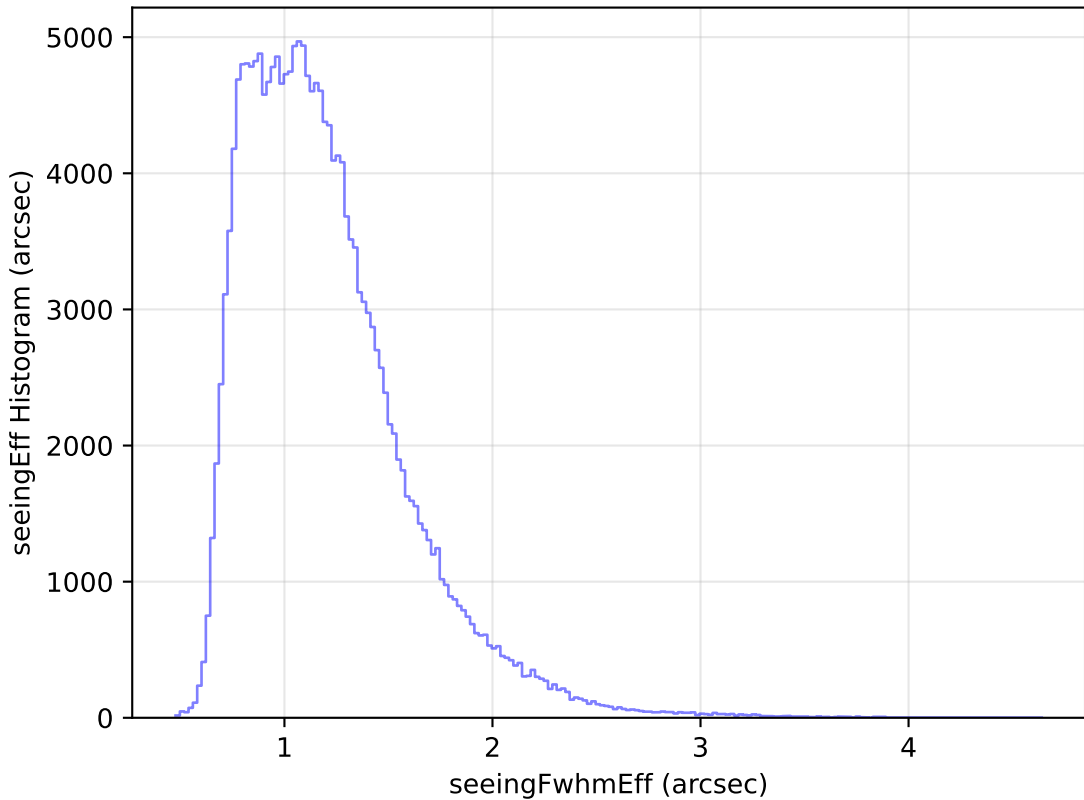
too_ignore_100_1v3.4_10yrs All sky g band: seeingEff Histogram
