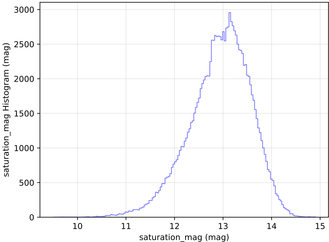
too_ignore_100_1v3.4_10yrs WFD u band: saturation_mag Histogram
