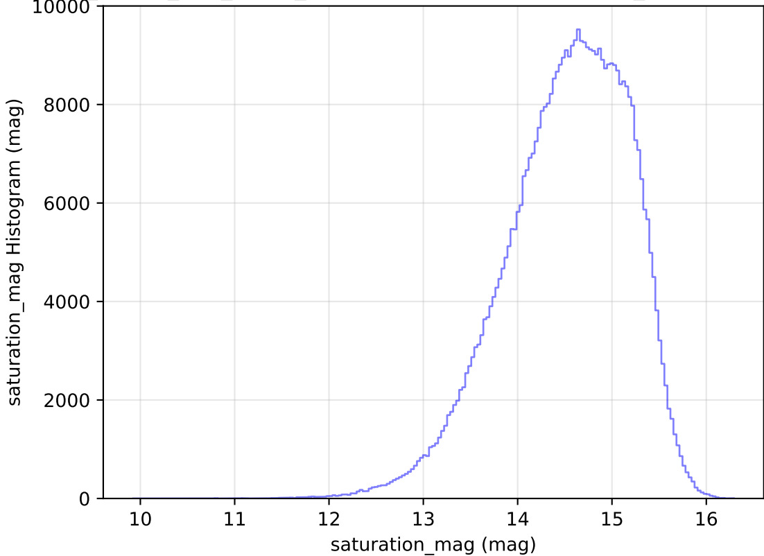
too_ignore_100_1v3.4_10yrs WFD r band: saturation_mag Histogram
