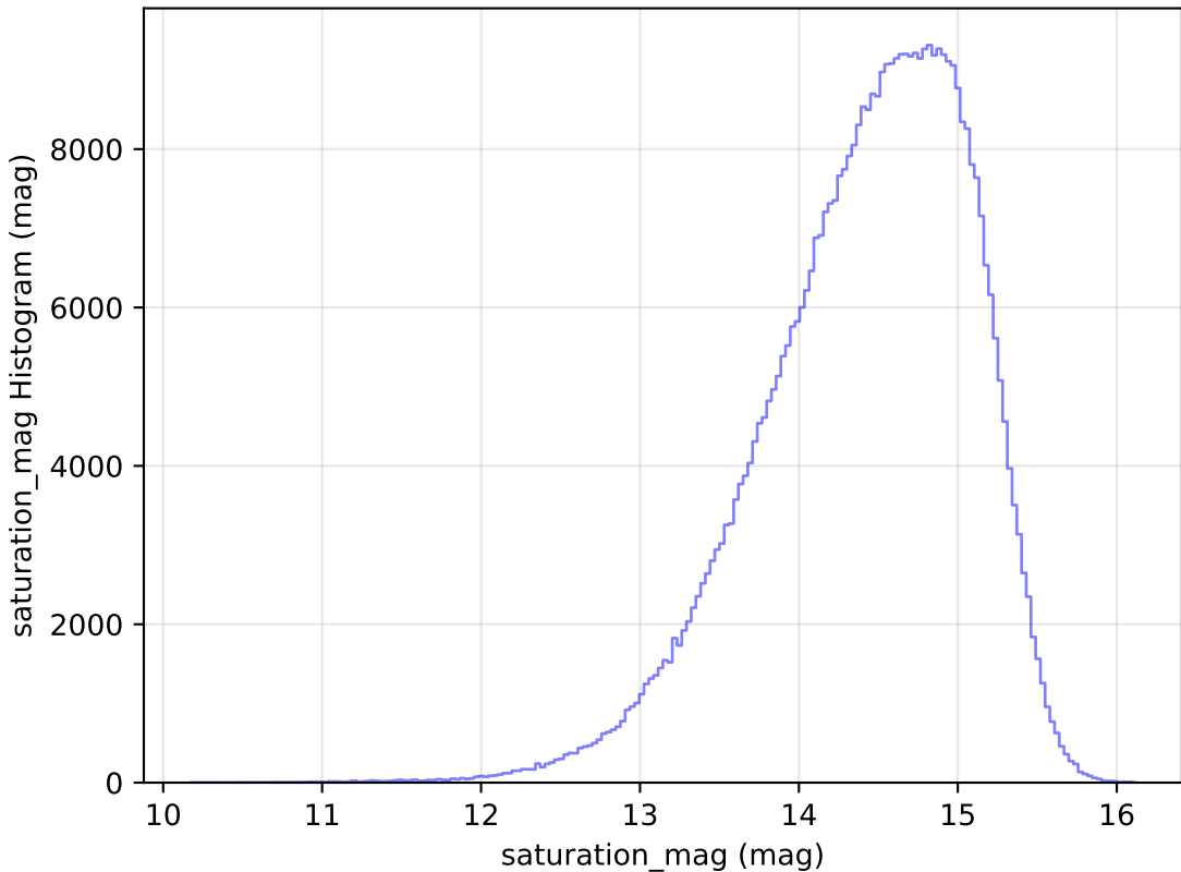
too_ignore_100_1v3.4_10yrs WFD i band: saturation_mag Histogram
