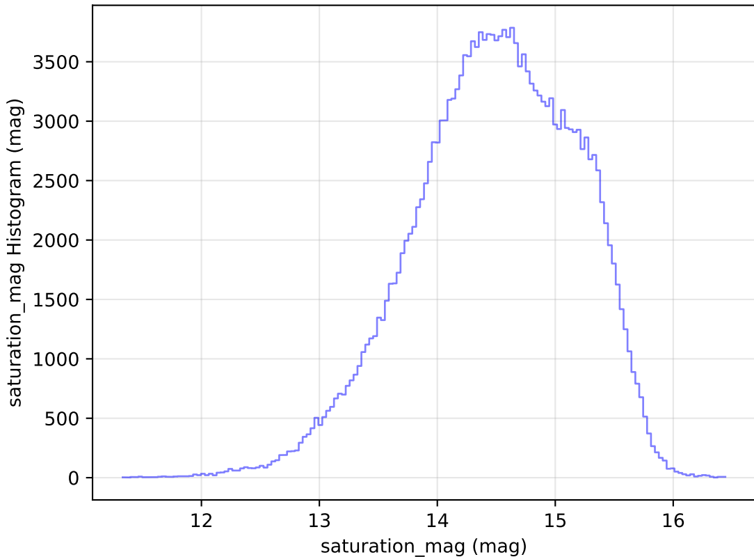
too_ignore_100_1v3.4_10yrs WFD g band: saturation_mag Histogram
