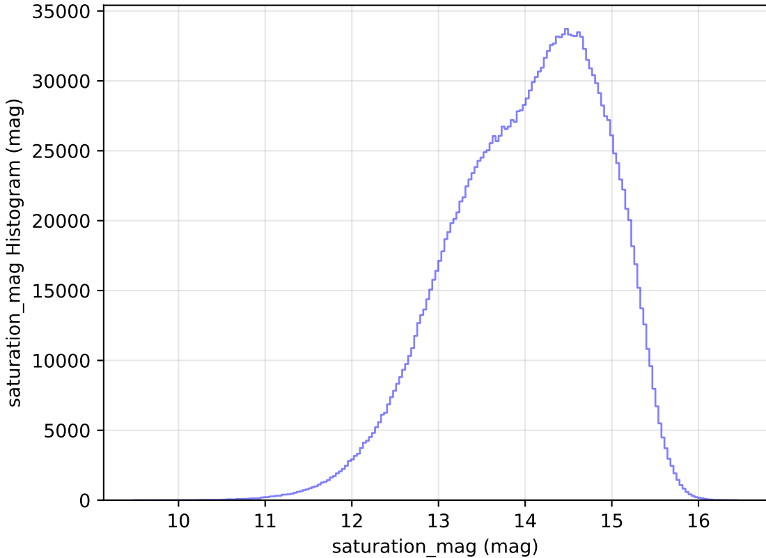
too_ignore_100_1v3.4_10yrs WFD all bands: saturation_mag Histogram
