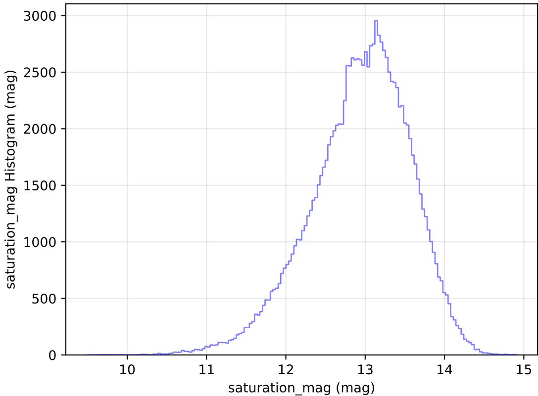
too_ignore_100_1v3.4_10yrs All sky u band: saturation_mag Histogram
