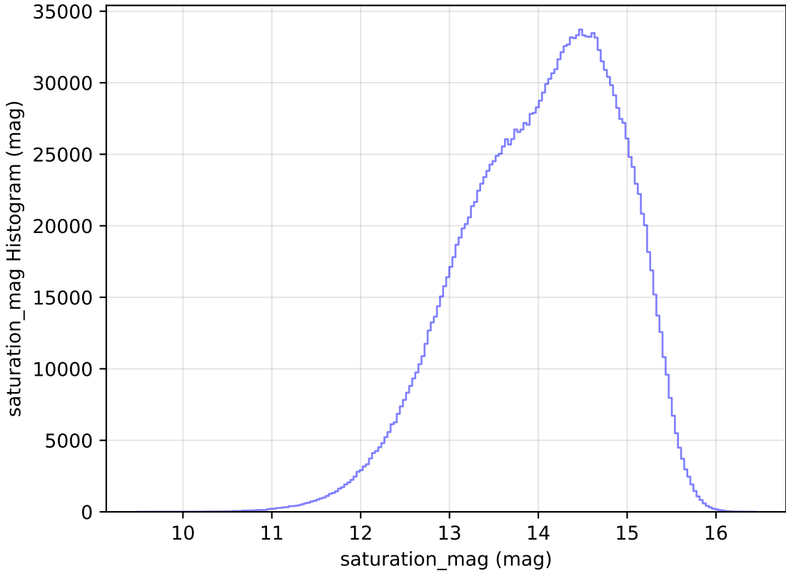
too_ignore_100_1v3.4_10yrs All sky all bands: saturation_mag Histogram
