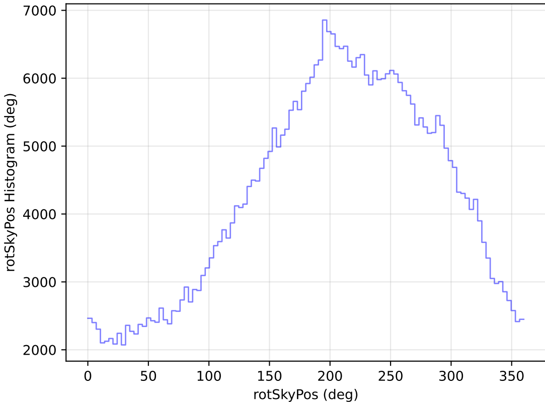
too_ignore_100_1v3.4_10yrs WFD z band: rotSkyPos Histogram
