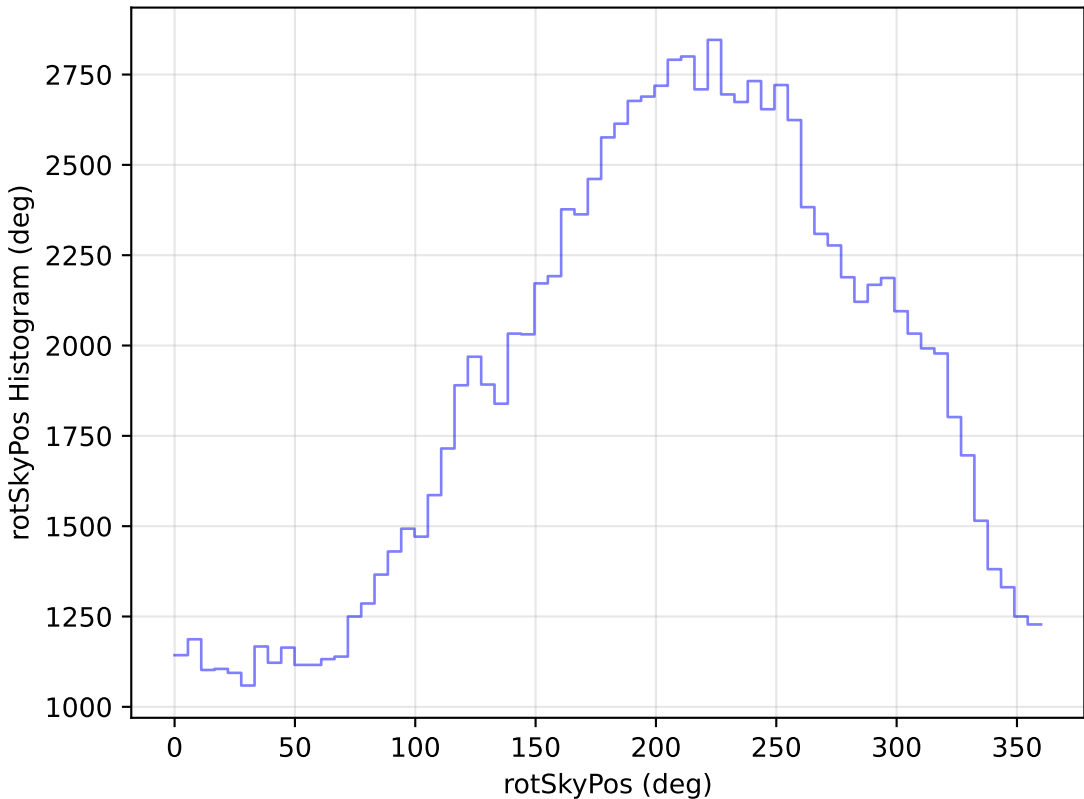
too_ignore_100_1v3.4_10yrs WFD u band: rotSkyPos Histogram
