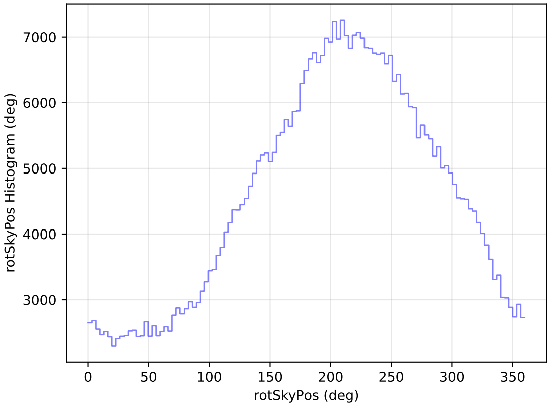
too_ignore_100_1v3.4_10yrs WFD i band: rotSkyPos Histogram
