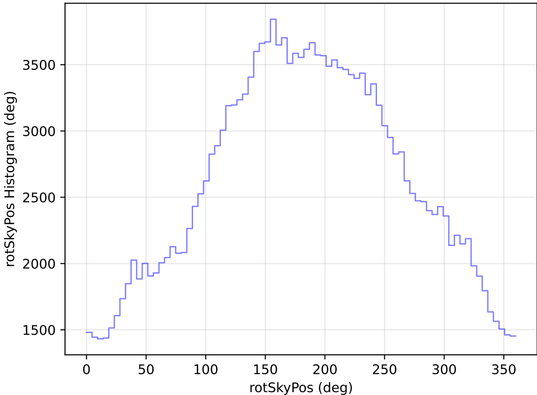
too_ignore_100_1v3.4_10yrs WFD g band: rotSkyPos Histogram
