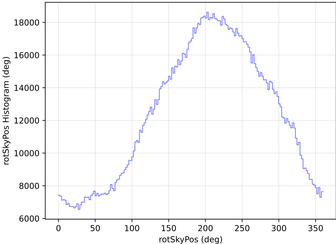
too_ignore_100_1v3.4_10yrs WFD all bands: rotSkyPos Histogram
