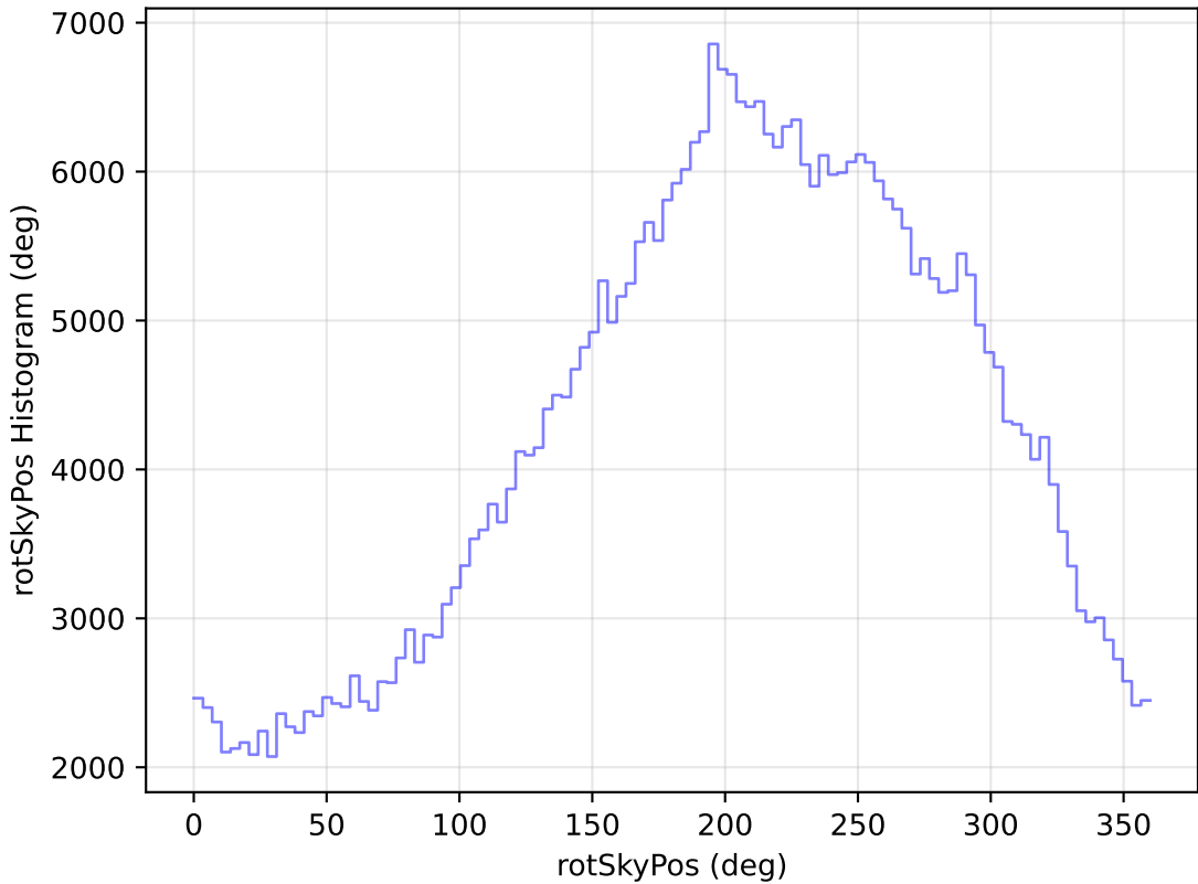
too_ignore_100_1v3.4_10yrs All sky z band: rotSkyPos Histogram
