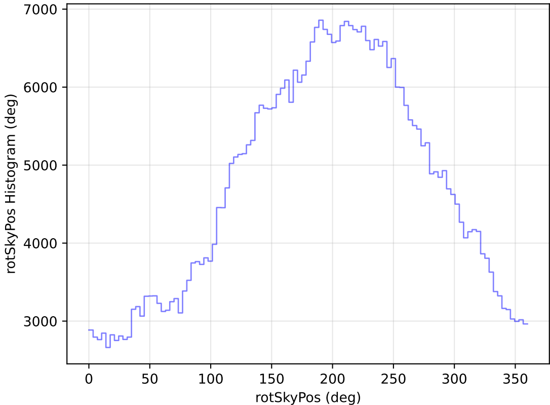
too_ignore_100_1v3.4_10yrs All sky r band: rotSkyPos Histogram
