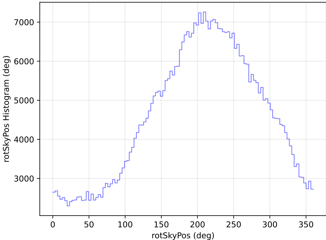
too_ignore_100_1v3.4_10yrs All sky i band: rotSkyPos Histogram
