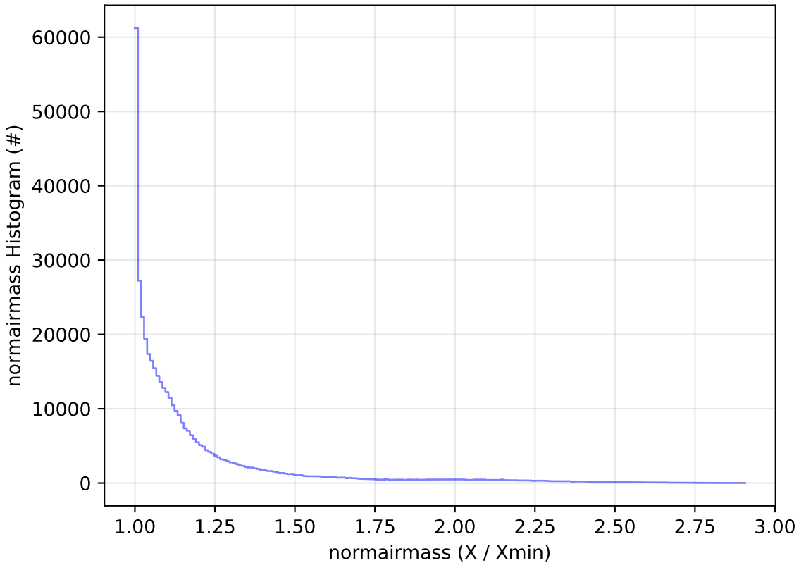
too_ignore_100_1v3.4_10yrs WFD z band: normairmass Histogram
