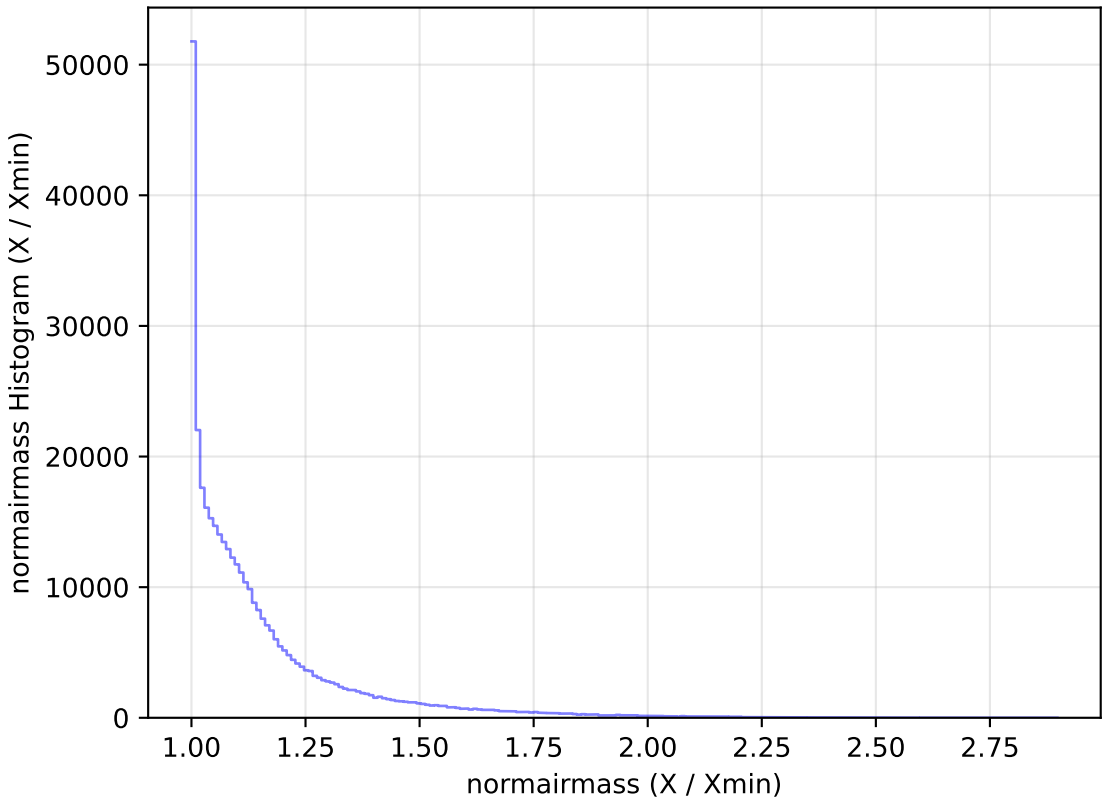
too_ignore_100_1v3.4_10yrs WFD y band: normairmass Histogram
