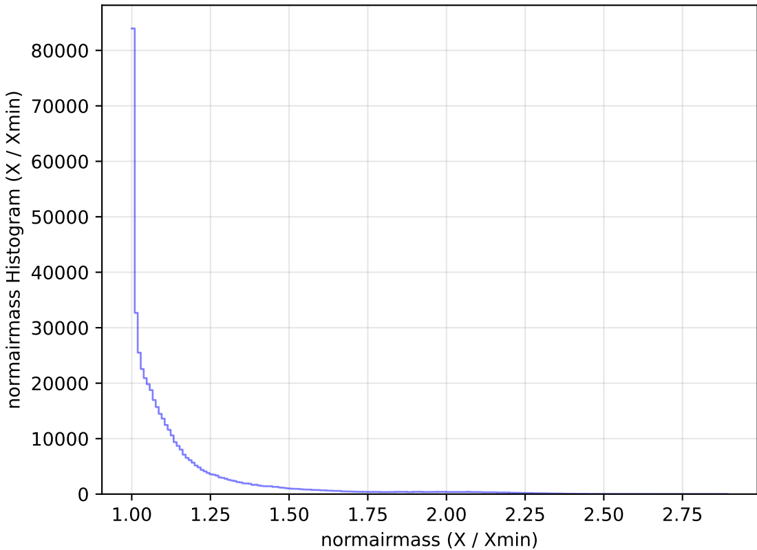
too_ignore_100_1v3.4_10yrs WFD r band: normairmass Histogram
