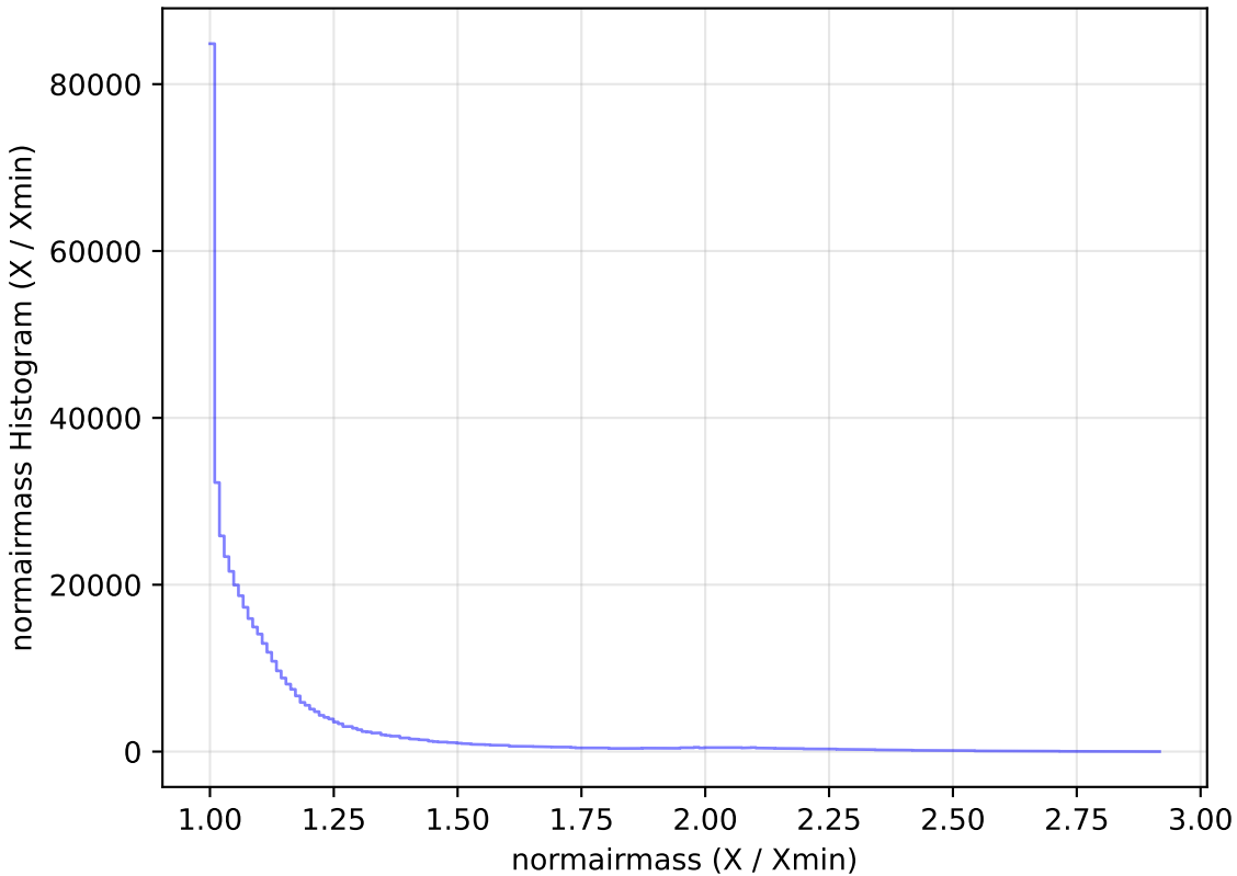
too_ignore_100_1v3.4_10yrs WFD i band: normairmass Histogram
