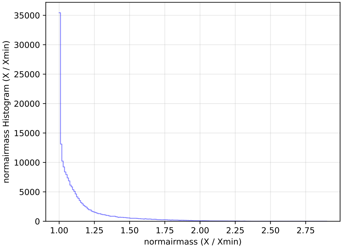
too_ignore_100_1v3.4_10yrs WFD g band: normairmass Histogram
