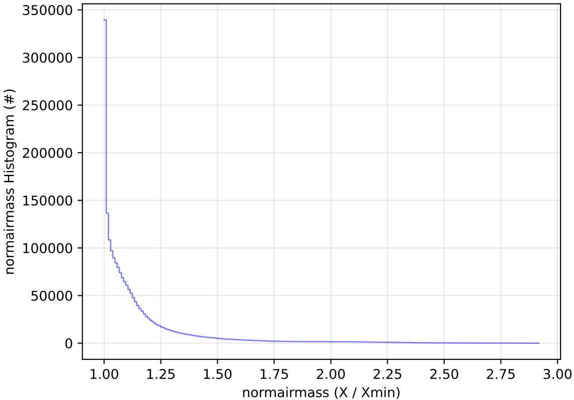
too_ignore_100_1v3.4_10yrs WFD all bands: normairmass Histogram
