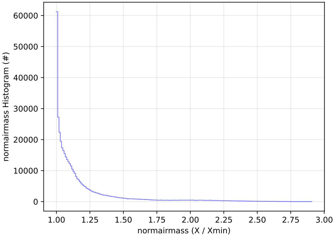
too_ignore_100_1v3.4_10yrs All sky z band: normairmass Histogram
