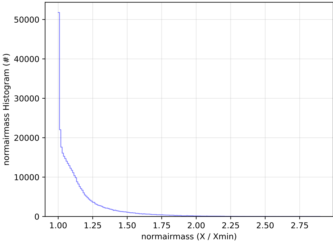
too_ignore_100_1v3.4_10yrs All sky y band: normairmass Histogram
