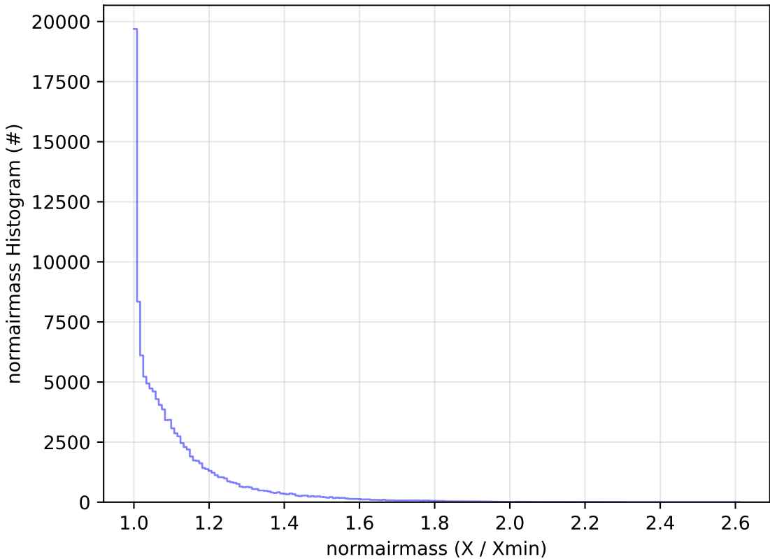
too_ignore_100_1v3.4_10yrs All sky u band: normairmass Histogram
