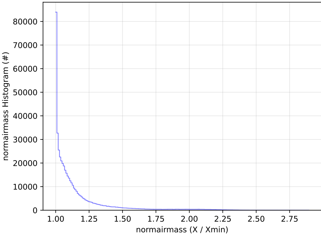
too_ignore_100_1v3.4_10yrs All sky r band: normairmass Histogram
