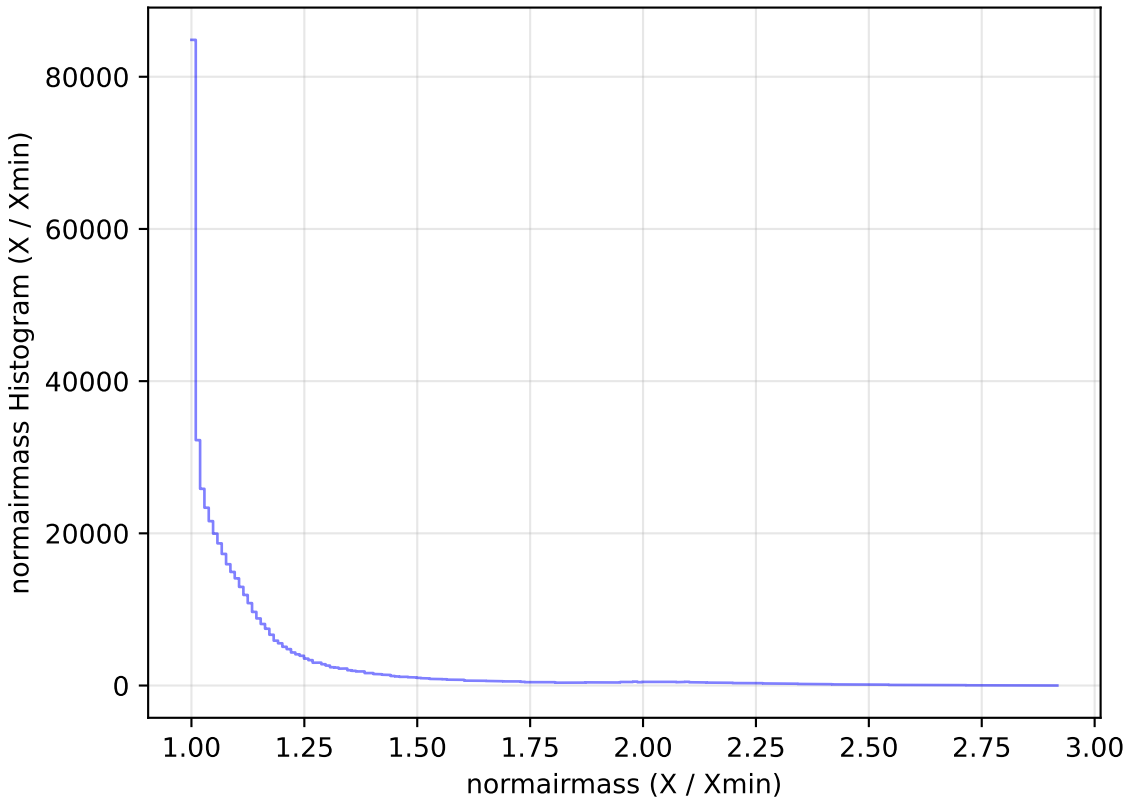
too_ignore_100_1v3.4_10yrs All sky i band: normairmass Histogram
