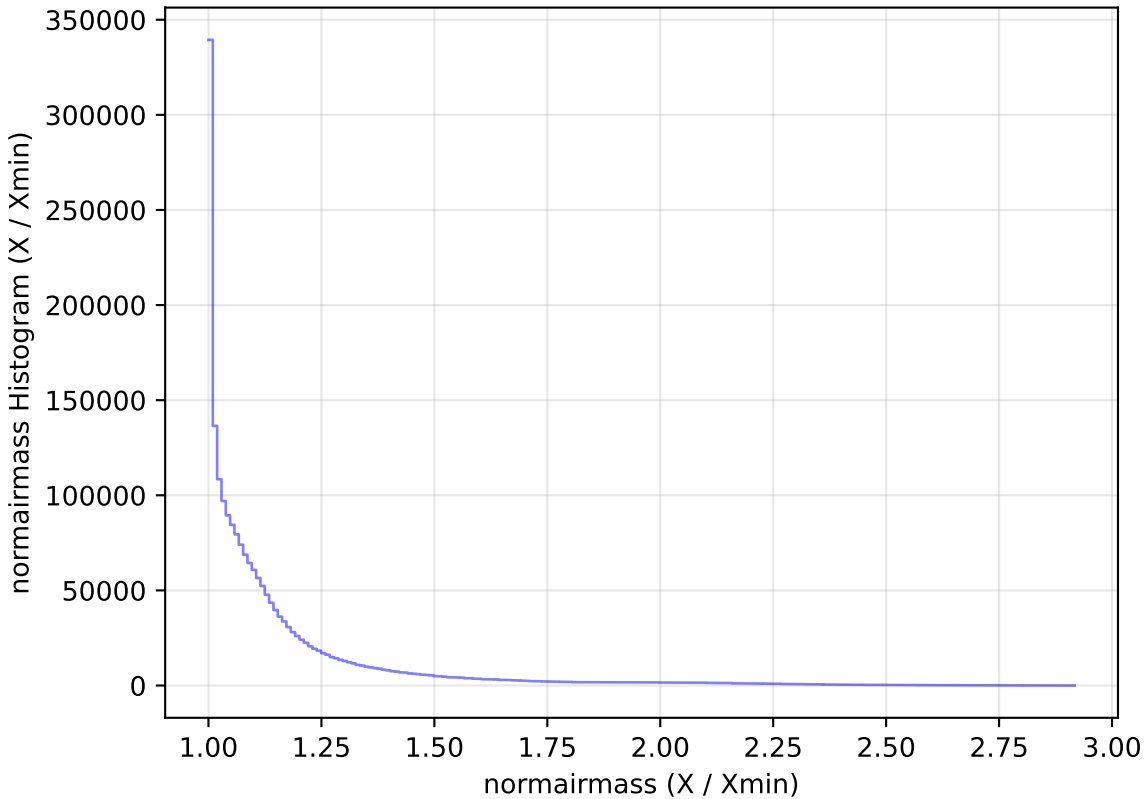
too_ignore_100_1v3.4_10yrs All sky all bands: normairmass Histogram
