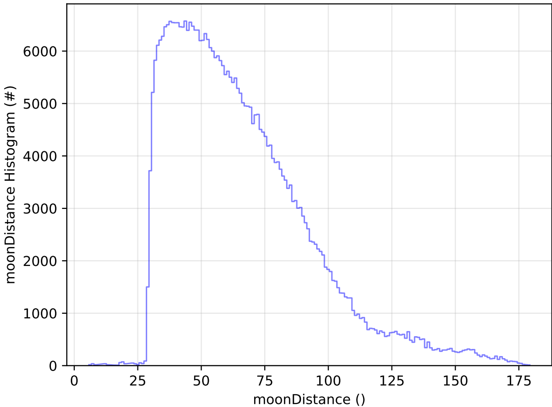
too_ignore_100_1v3.4_10yrs WFD y band: moonDistance Histogram
