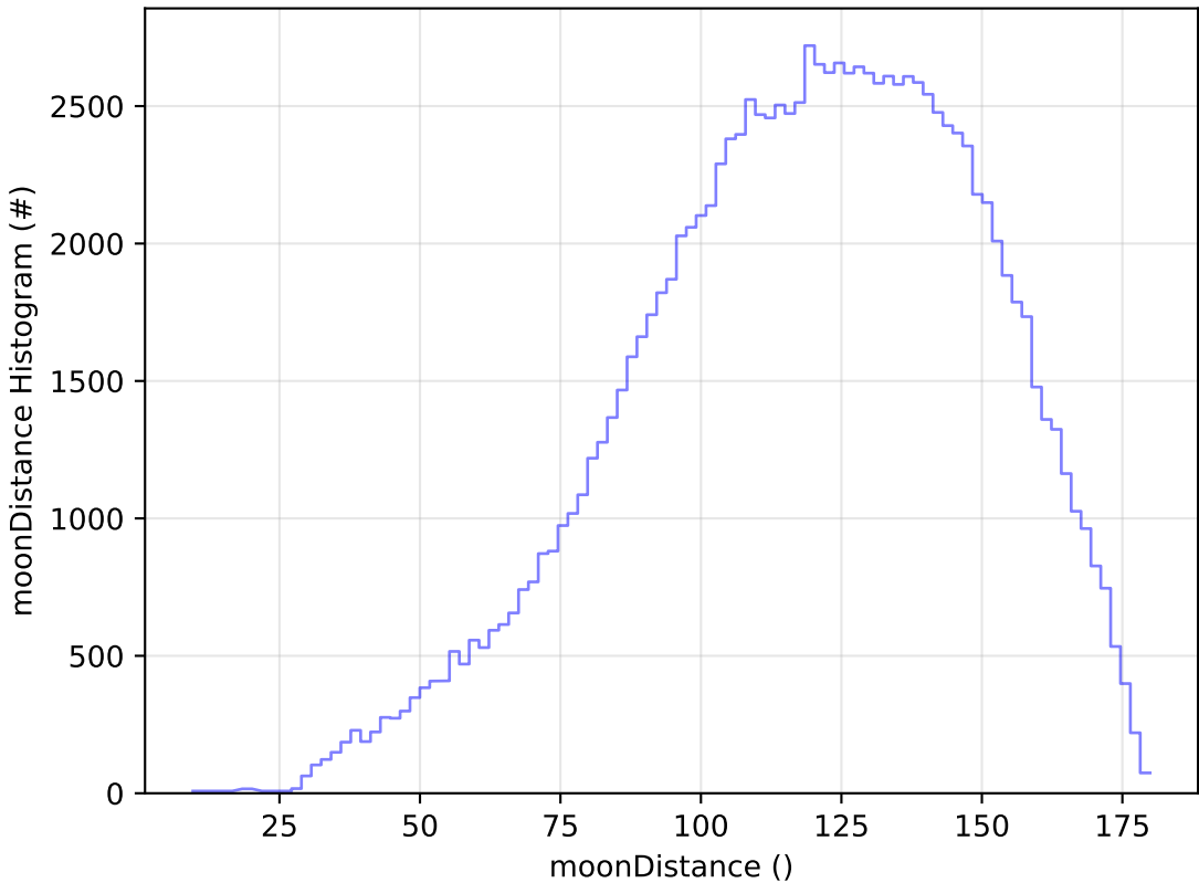
too_ignore_100_1v3.4_10yrs WFD u band: moonDistance Histogram
