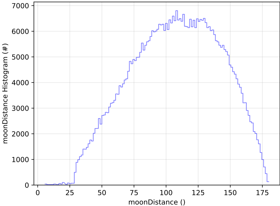
too_ignore_100_1v3.4_10yrs WFD r band: moonDistance Histogram
