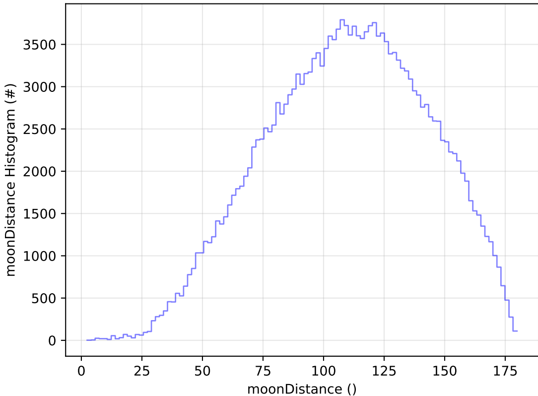
too_ignore_100_1v3.4_10yrs WFD g band: moonDistance Histogram
