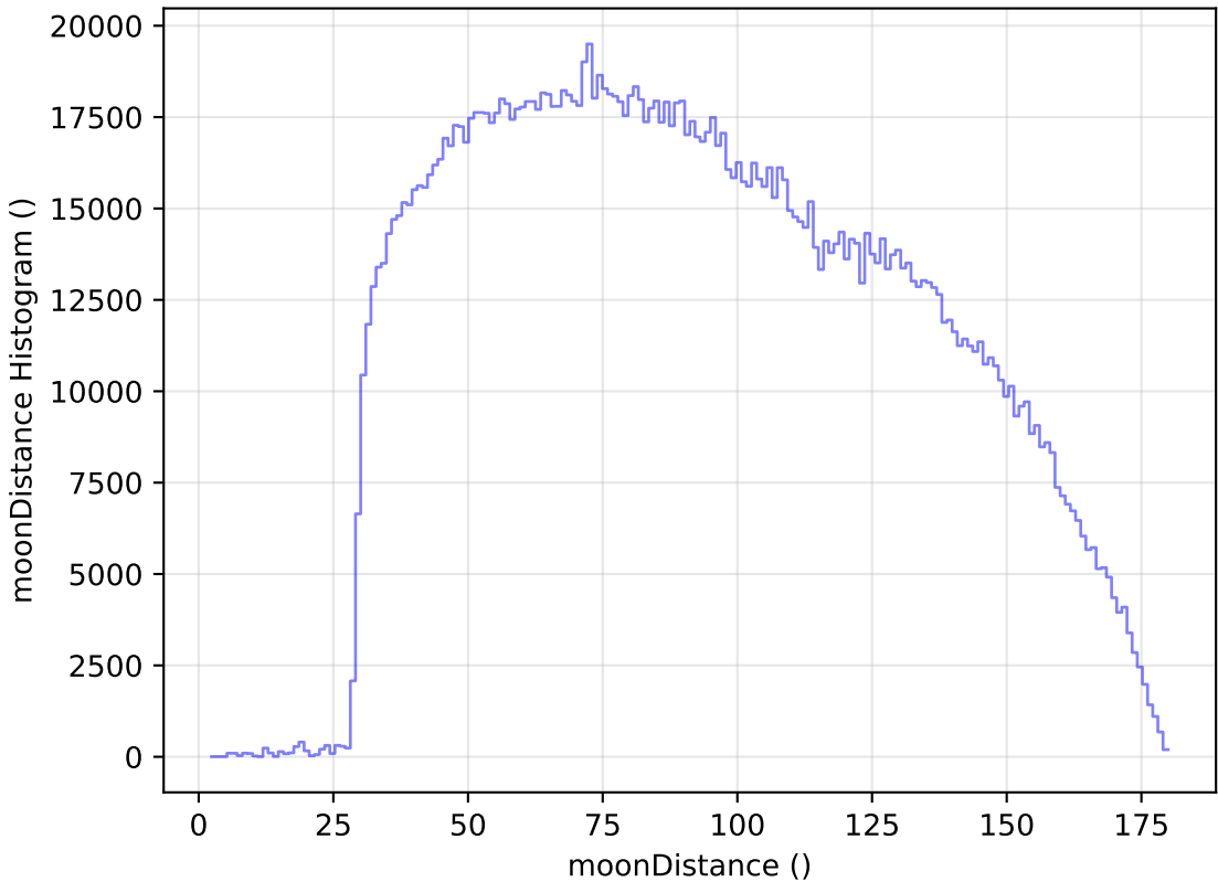
too_ignore_100_1v3.4_10yrs WFD all bands: moonDistance Histogram
