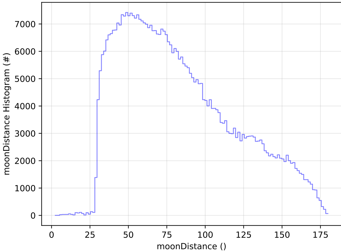
too_ignore_100_1v3.4_10yrs All sky z band: moonDistance Histogram
