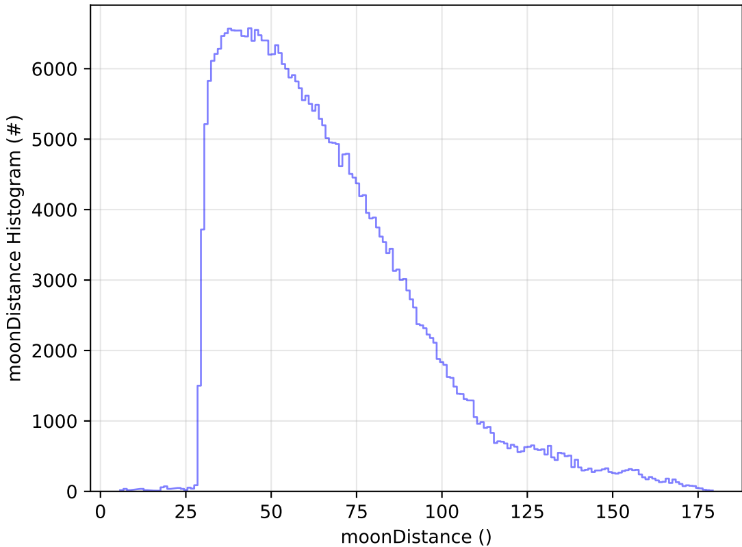
too_ignore_100_1v3.4_10yrs All sky y band: moonDistance Histogram
