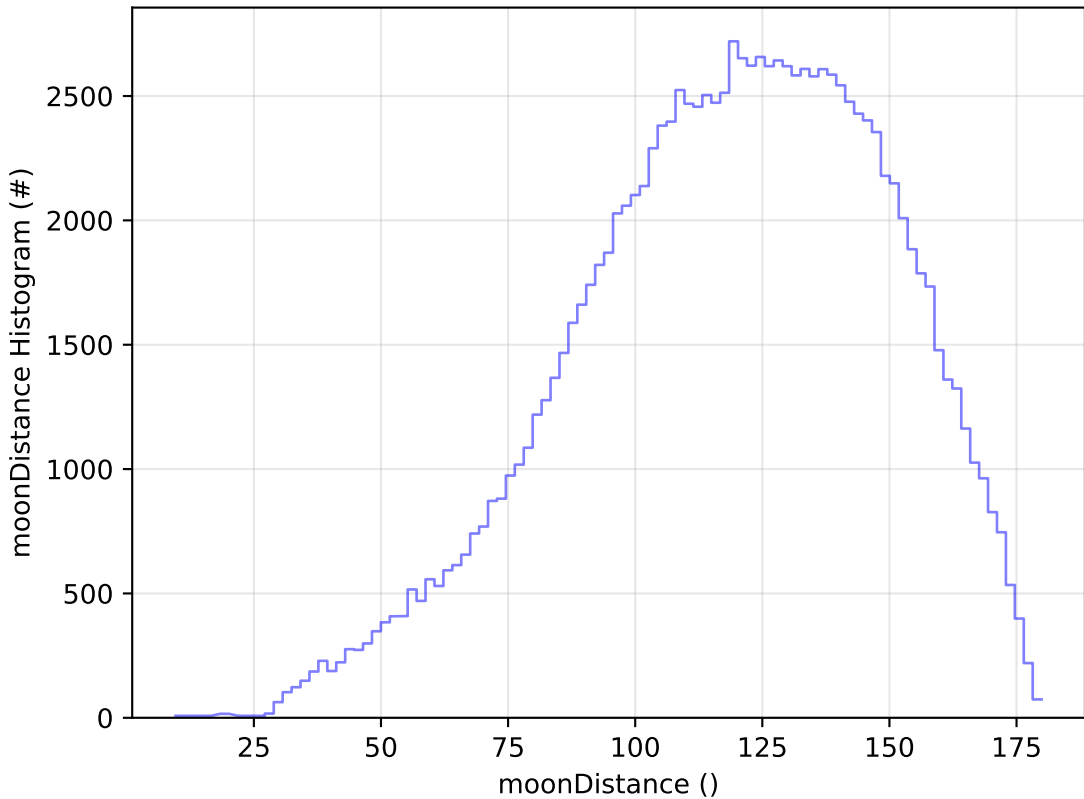
too_ignore_100_1v3.4_10yrs All sky u band: moonDistance Histogram
